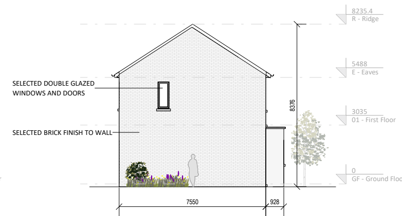
5 H07A Left Elevation 1 : 200
